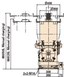
CE-R-1D (25L)
