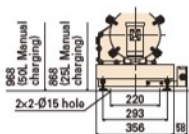
CE-R-1D (25L)
