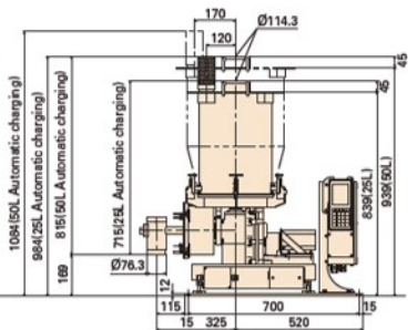
CE-R-2D-MP(50L)
