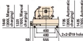
CE-R-3D (100L)
