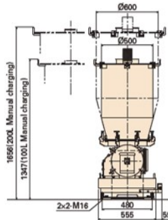
CE-R-3D (100L)
